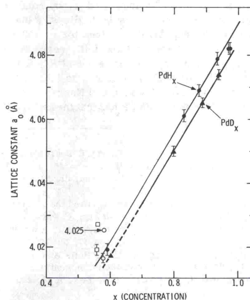
FIG. 1. Lattice constants versus concentration for \beta -PdH _x and \beta -PdD _x at 77 K. The upper line passes through values for \beta -PdH _x while the lower line passes through those for \beta -PdD _x . Previously accepted room-temperature \beta_{\min} values for PdD _x and PdH _x are shown as an open square and circle, respectively; the 77-K values were obtained by subtracting \Delta (see text) and are shown as an open square and circle with error limits similar to those we experienced in our measurements. Solid triangle gives our PdD _x value (4.016 Å) at 77 K provided it would lie on the line extended from our higher x values. Our sample of PdH _x prepared at 20-Torr pressure yielded a_0 = 4.028 and 4.019 Å for room temperature and 77 K, respectively; this sample might contain at most 5% of the \alpha phase.
